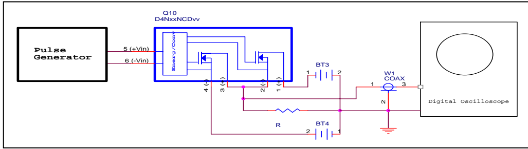
Figure 5 Set-up for test of a SPDT hook-up
